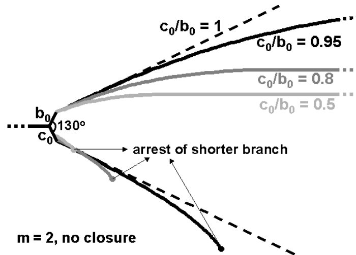
Figure 5 – Bifurcated crack paths for several c_0/b_0 ratios.
