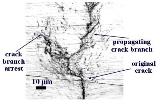
Figure 6 – Crack branching on an SAE 4340 ESE(T) specimen.
