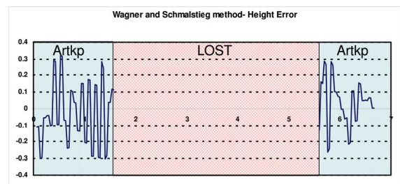
Figure 5: Graph of error (meter) vs time(second) using Wagner and Schmalstieg’s [15] approach (Artkp means ARToolKitPlus)
