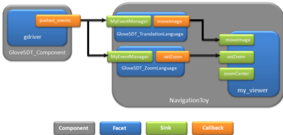
Fig. 1. OpenInterface pipeline.
