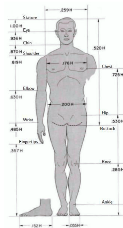
Figure 5: Body segment lengths expressed as a percentage of height [23]
